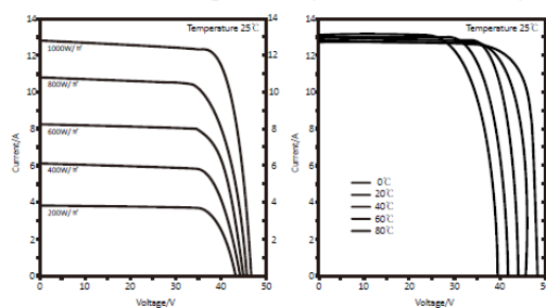
Current-Voltage Curve (BSM500PM5-78SA)
